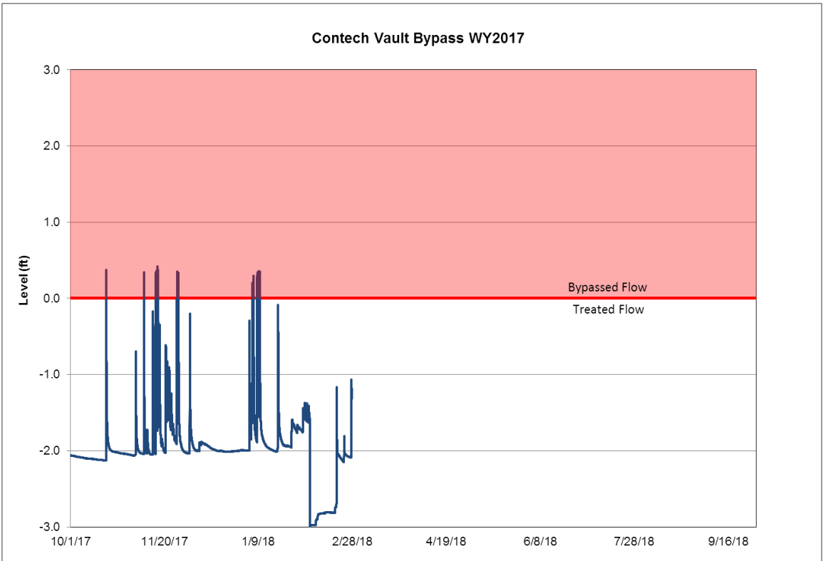
Figure 5: Bypassed flow in Contech MFS vault, fall/winter WY18
