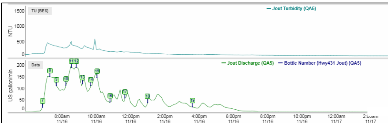
Figure 10: Hydrograph, continuous turbidity and sample distribution at the Jellyfish Outflow for the 11/16/17 rain event.
