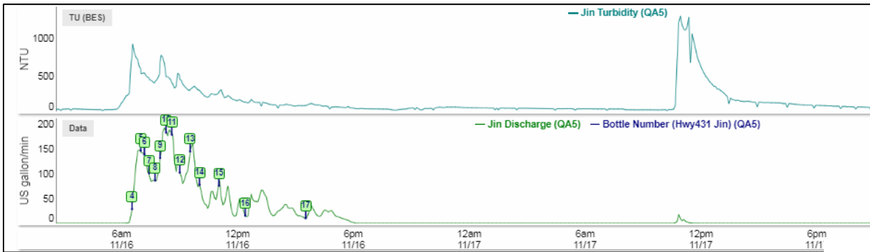
Figure 9: Hydrograph, continuous turbidity and sample distribution at the Jellyfish Inflow for the 11/16/17 rain event.
