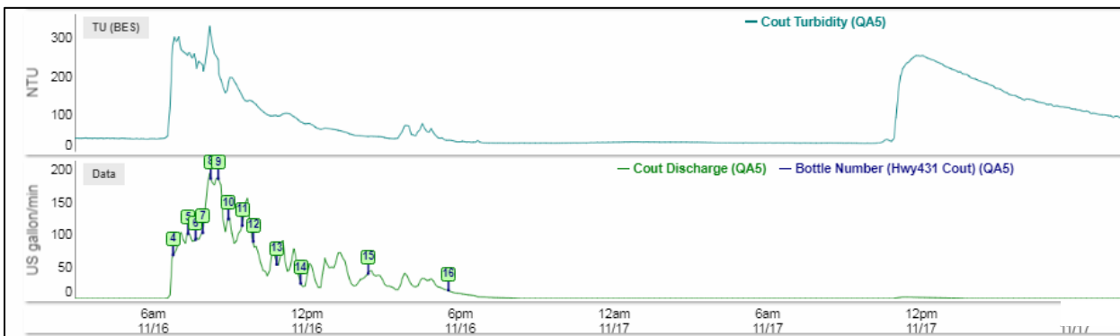
Figure 8: Hydrograph, continuous turbidity and sample distribution at the Contech MFS Outflow for the 11/16/17 rain event.
