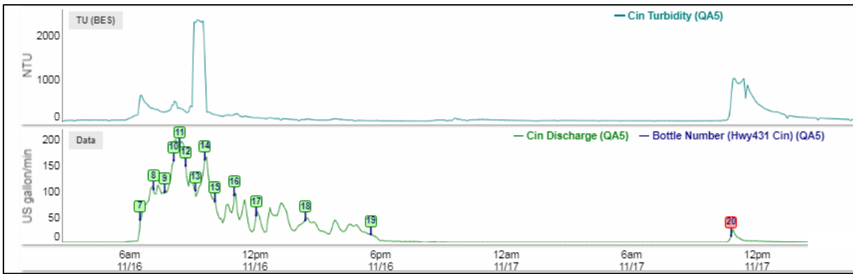
Figure 7: Hydrograph, continuous turbidity and sample distribution at the Contech MFS Inflow for the 11/16/17 rain event
